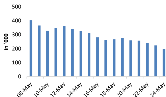
Daily Additions in Covid Cases in India (Source: Covid19)
